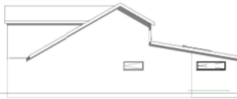
East Elevations Proposed
